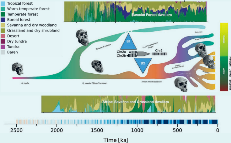
Figure 31. Schematic of phylogenetic tree of human species and biome preferences of Eurasian (upper) and African (lower) populations.
