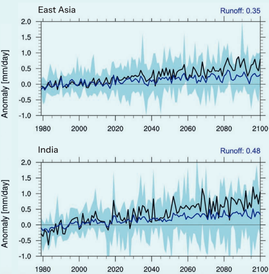
Figure 15. Time series of summer anomalous precipitation (PR, black) and runoff (blue) averaged over East Asia and India during the period from 1979 to 2100. Blue shading represents the minimum and maximum anomalous runoff among seven CMIP6 models.
