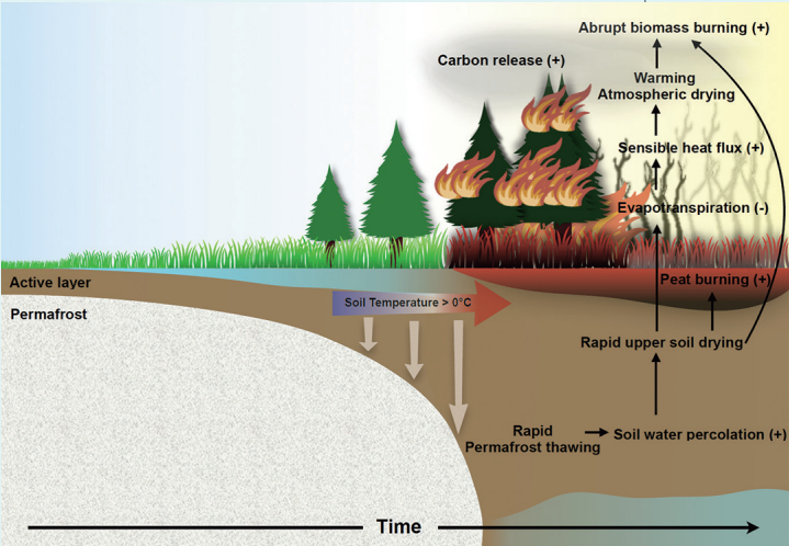
Figure 25. Schematic diagram highlighting pathways for an abrupt increase in wildfires following permafrost thaw.
